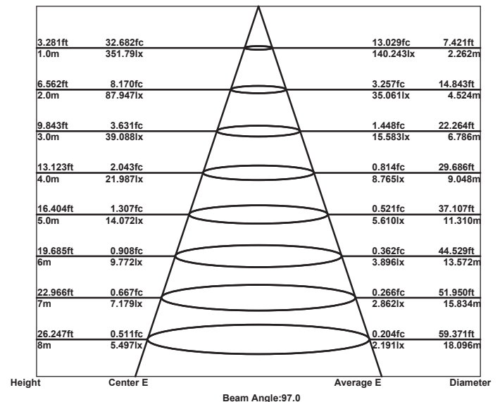
Illuminance-Distance Curve
