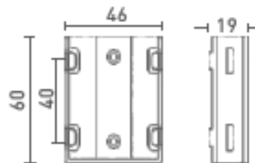
Remote holder
