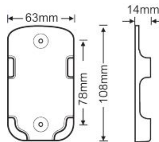
Remote holder
